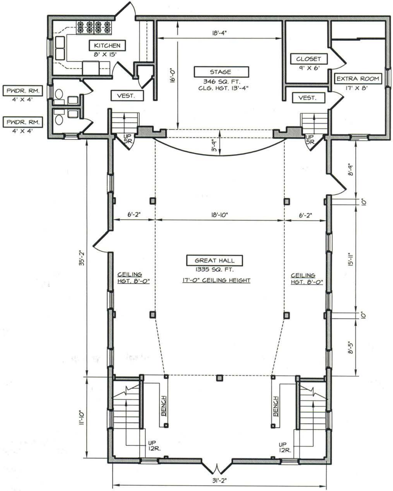
① FLOOR PLAN 1/8" = 1'-0"
